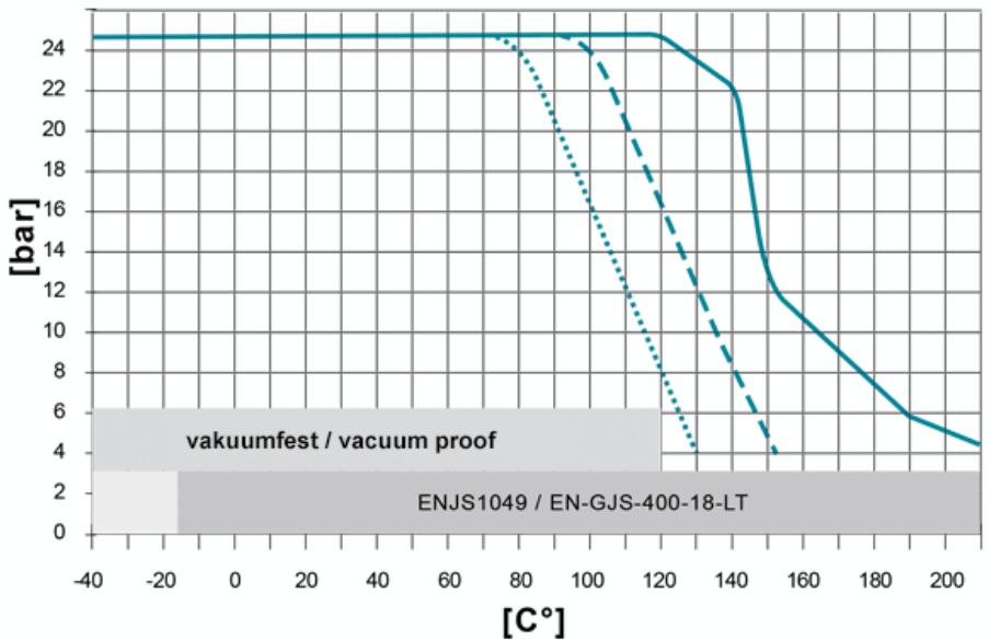
General Pressure-Temperature-Diagram
